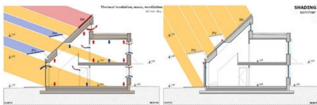
Solar active house, use of solar radiation [7.11]
