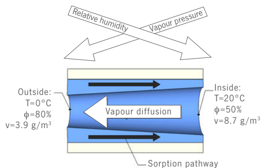
Moisture transport in wood [7.4]
