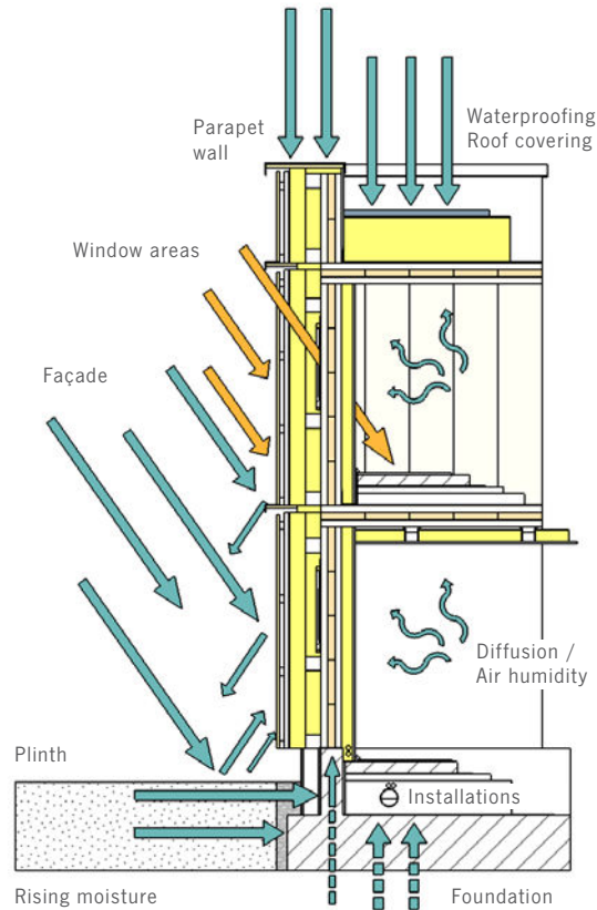
Effects on the façade
