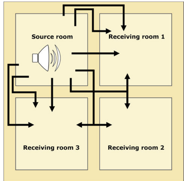
Secondary sound paths of airborne sound transmission
