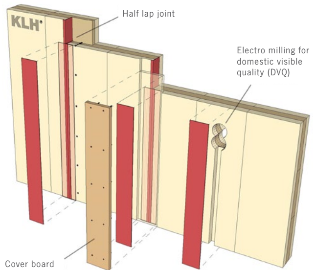
SCHEMATIC CONNECTION
