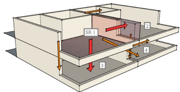
Typical transmission paths to other units
